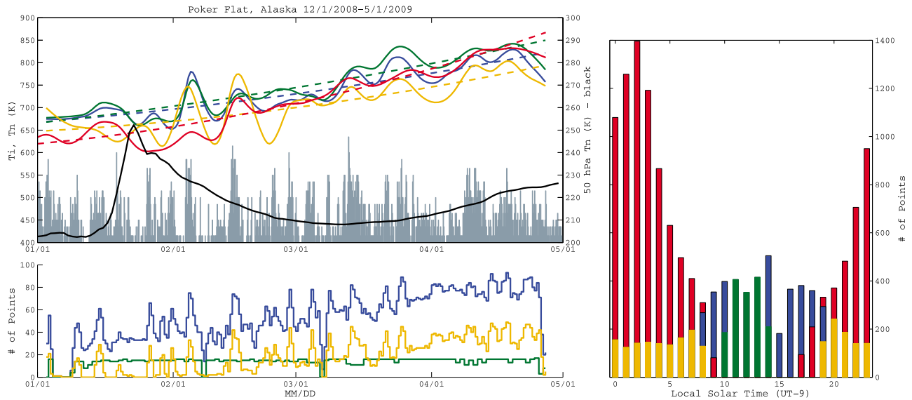
Figure 8. (top left) Smoothed versions of PFISR T_i binned in three time periods: all data (blue), 1000–1400 LST (green), 1900–0800 LST (brown). The red curve is a smoothed version of the FPS T_n . (bottom Left) Number of points for each curve in a given 24 h period for the time series. (right) Histogram of data points in local time.
